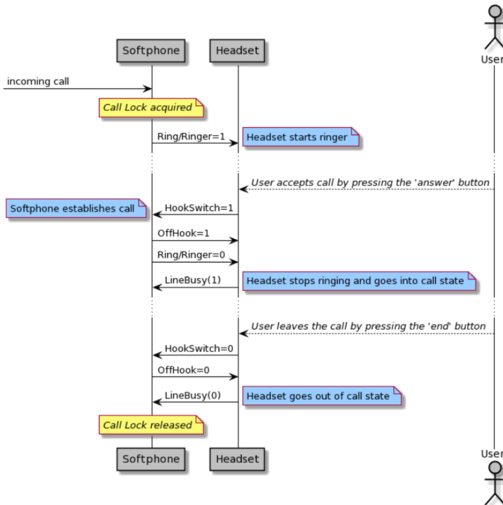
Figure 4 Sequence diagram: Incoming call accepted and ended on the device.
