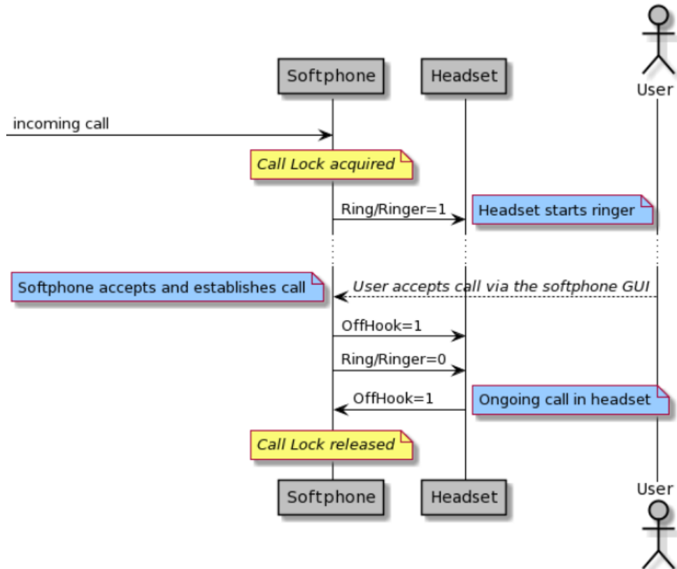
Figure 5 Sequence diagram: Incoming call accepted on softphone GUI.
