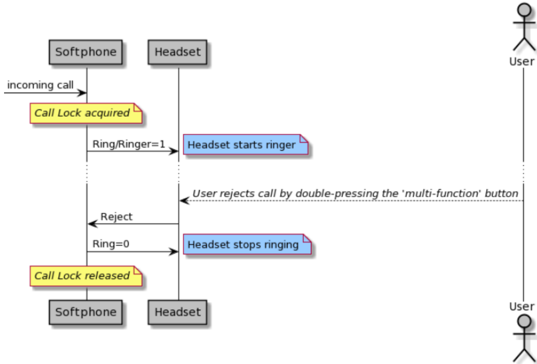
Figure 6 Sequence diagram: Incoming call rejected on the device.
