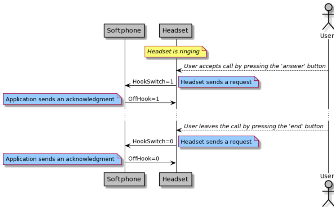
Figure 3 Example of simplified off-hook/on-hook sequence diagram (illustrative purpose only).
